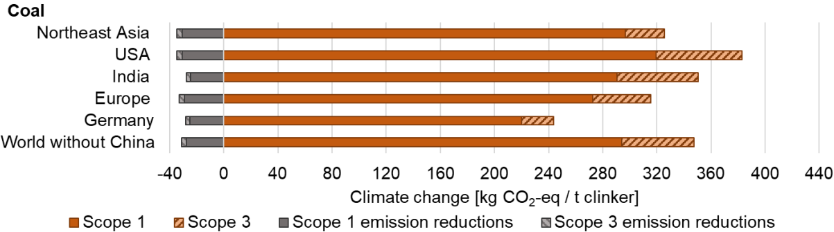
Figure 9 Impact of hard coal reduction on GHG emissions. The results refer to the fuel efficiency achieved at a first pilot plant after a four month operation period.
