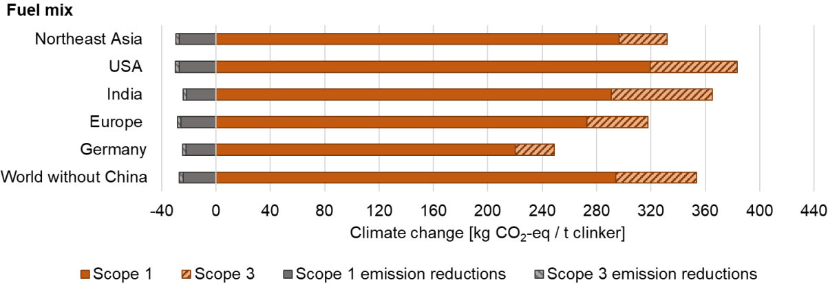
Figure 8 Impact of fuel mix reduction on GHG emissions. The results refer to the fuel efficiency achieved at a first pilot plant after a four month operation period.
