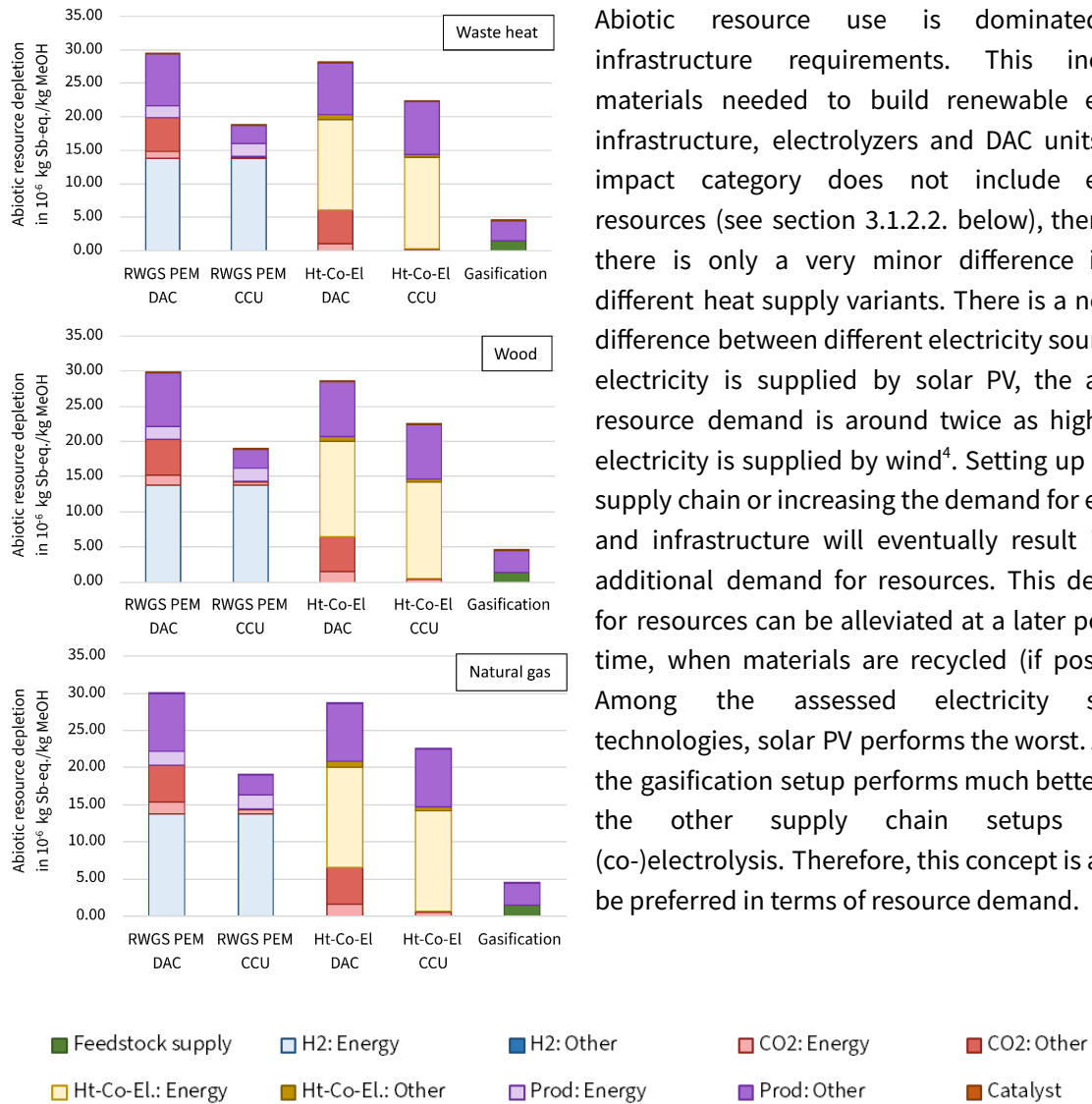
Figure 3 Abiotic resource depletion of green methanol production. The diagrams show the same supply variants and energy supply scenarios as depicted in Figure 2. Abbr.: DAC - Direct air capture, GHG - Greenhouse gas, Ht-Co-El. - High-temperature co-electrolysis, MeOH - Methanol, PEM - Proton exchange membrane.
