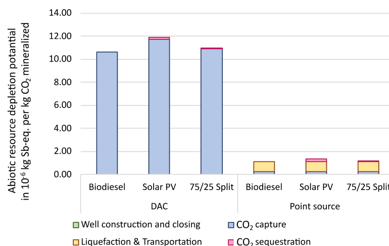
Figure 5 Abiotic resource demand (abiotic resource depletion) of carbon capture and mineralization in 10^{-6} kg Sb-eq. per kg CO 2 permanently sequestered in Peridotite formations. Abbr.: DAC - Direct air capture, PV - photovoltaics.
