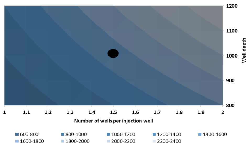
Figure 2 Total well depth as a function of well depth and number of wells required per injection well. The black circle marks the targeted depth and number of observation wells per injection well needed.
