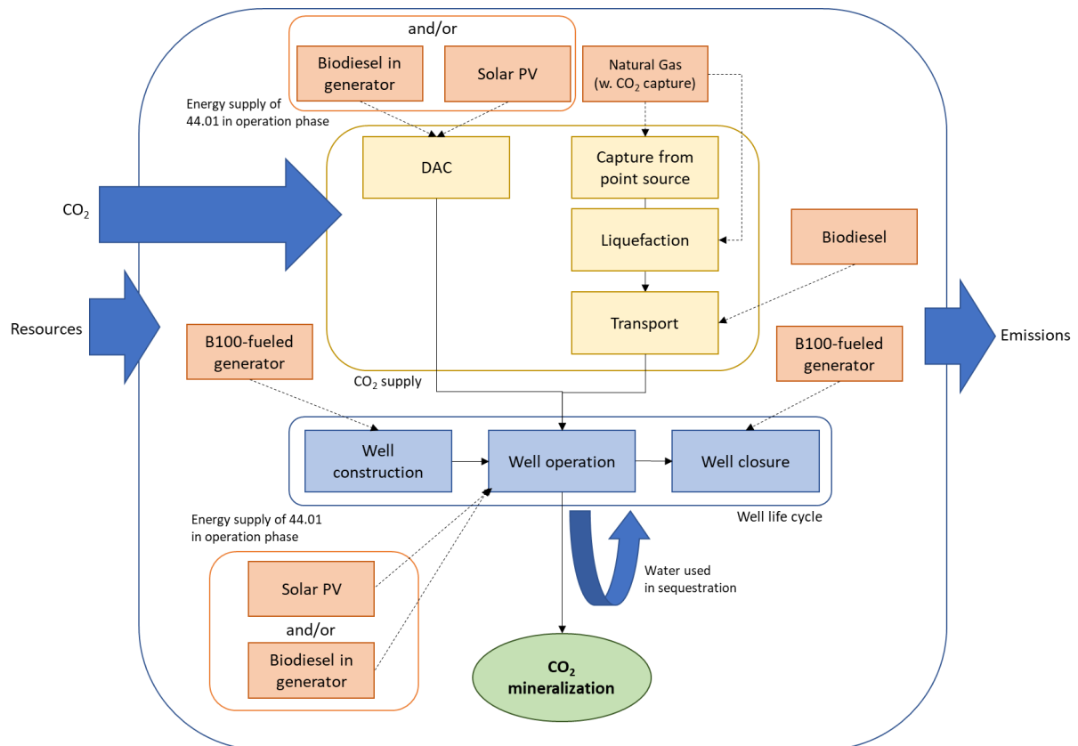
Figure 1 Depiction of system boundaries. Different supply chains for the provision of carbon dioxide are assessed: DAC and capturing from a point source (a natural gas power plant). Energy supply is depicted by orange boxes. Background processes, e.g. raw material supply, infrastructure, waste treatment, etc. are included in the assessment but not depicted in the figure. Water used in sequestration is fed back into the aquifer from which it was taken. Therefore water does not leave the catchment area. Diesel-fueled machinery operates with biodiesel (B100). Abbr.: DAC - Direct air capture, PV - photovoltaics.
