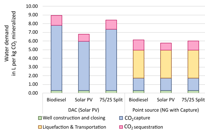
Figure 7 Water use of carbon capture and mineralization in L per kg CO 2 permanently sequestered in Peridotite formations. Abbr.: DAC - Direct air capture, PV - photovoltaics.
