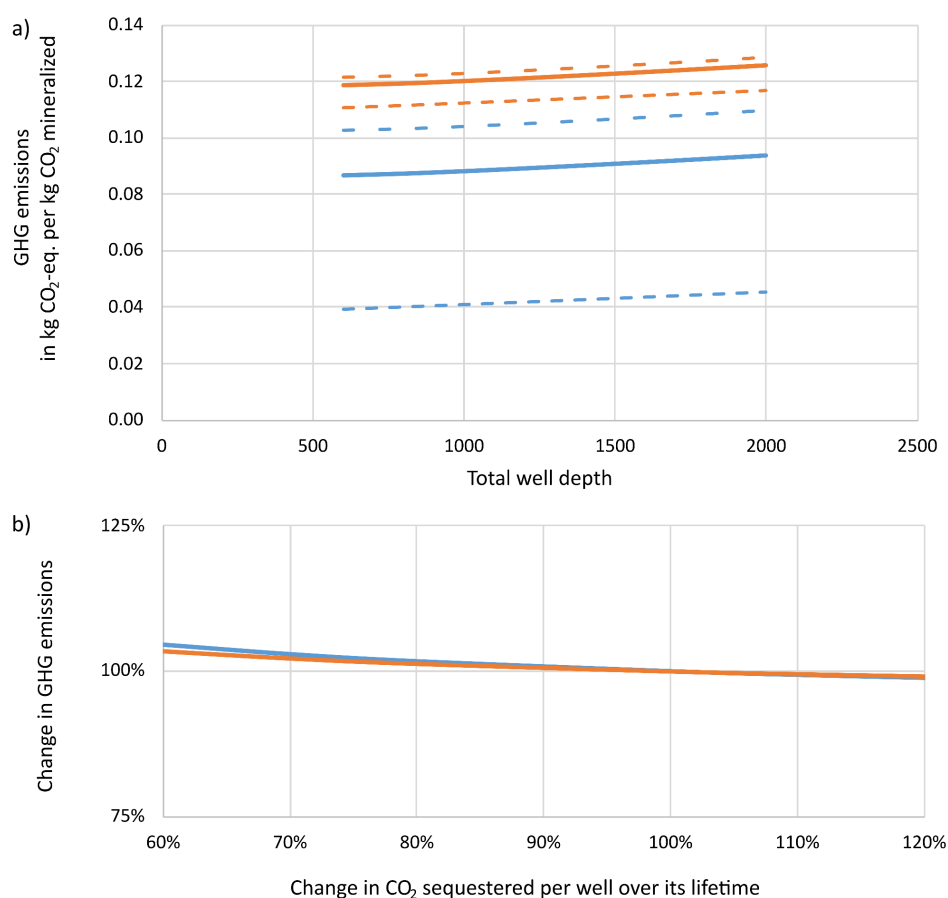
Figure 4 Sensitivity analyses: dependence of results on the total well depth (a), and the total quantity of CO 2 that can be mineralized with a single well over its lifetime (b). Abbr.: DAC - Direct air capture, GHG - Greenhouse gas, PV - photovoltaics.
