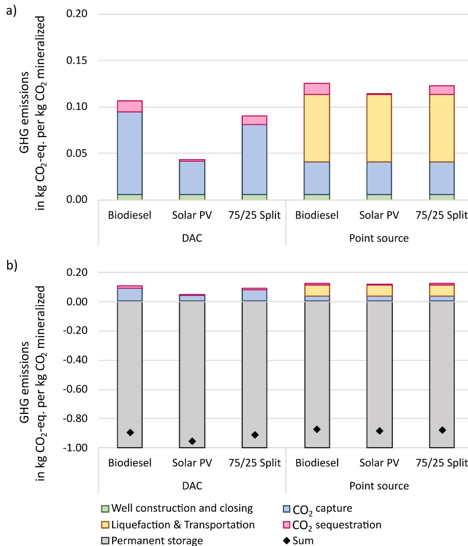
Figure 3 GHG emissions of carbon capture and mineralization in kg CO 2 -eq. per kg CO 2 permanently sequestered in Peridotite formations without (a) and with (b) the consideration of the CO 2 mineralization, i.e. -1 kg CO 2 per kg CO 2 sequestered. Abbr.: DAC - Direct air capture, GHG - Greenhouse gas, PV - photovoltaics.
