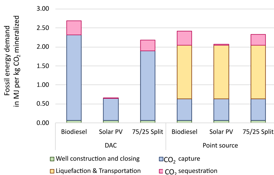
Figure 6 Fossil energy demand of carbon capture and mineralization in MJ per kg CO 2 permanently sequestered in Peridotite formations. Abbr.: DAC - Direct air capture, PV - photovoltaics.
